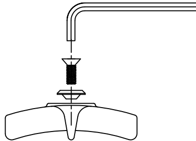
VANDAL PROOF KIT USED WITH T&S 4-ARM HANDLES
