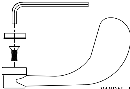
VANDAL PROOF KIT USED WITH T&S 4" OR 6" WRIST ACTION HANDLES
