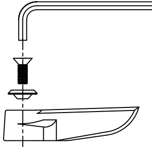
VANDAL PROOF KIT USED WITH T&S LEVER HANDLES
