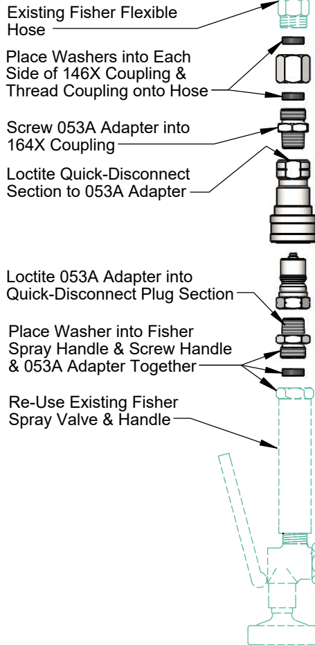
To Retro-Fit a Fisher Pre-Rinse Unit
